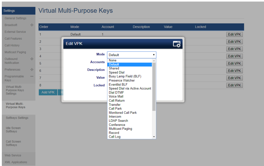
Figure 15: Edit VPK - Fixed VPK
